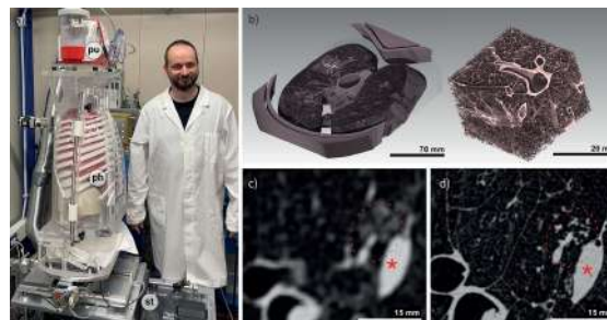
Lung imaging setup at the SYRMEP beamline, including the specially-designed positioning stage and resulting higher resolution. Figure from Dullin et al., European Respiratory Journal, 2024. CC BY 4.0 .
